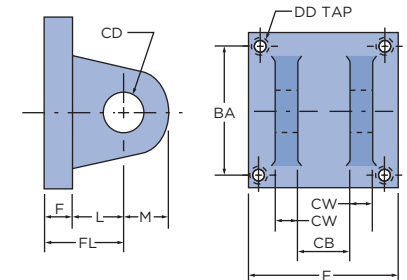
CLEVIS BRACKET
