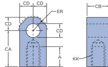
CLEVIS BRACKET
